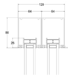
top rail
