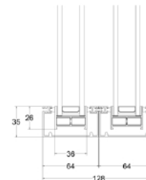
bottom rail
